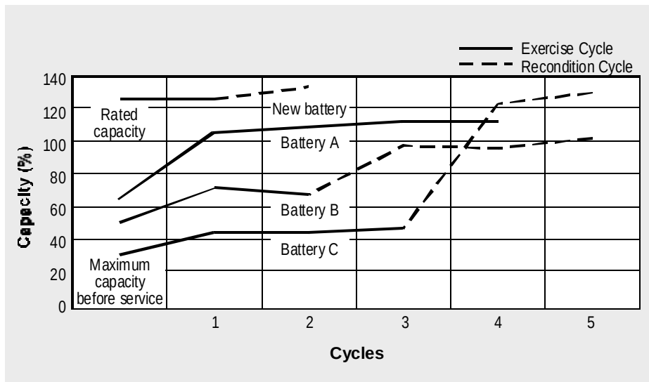
Figure 3: Effects of exercise and recondition.
