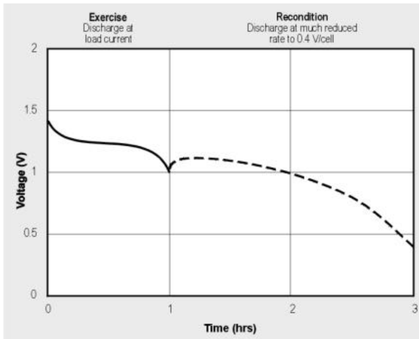
Figure 2: Exercising and reconditioning batteries on a Cadex battery analyzer.
